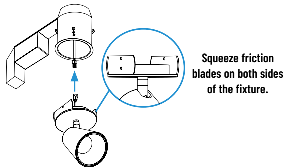
Connect luminaire and install
